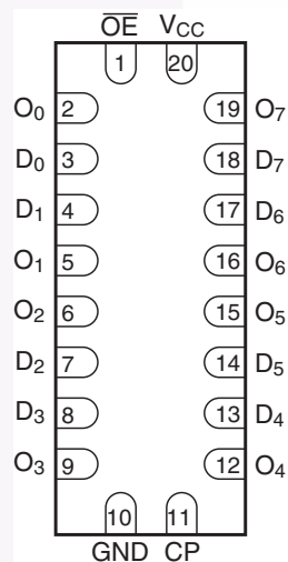
Pad Assignments for DQFN
