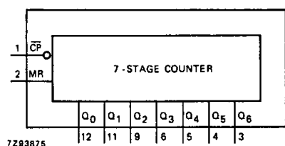
Fig. 4 Functional diagram.
