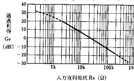
通過利得対入力直列抵抗特性例 ( f = 1\text{kHz}, R_L = 10\text{k}\Omega, T_a = 25^\circ\text{C} )
