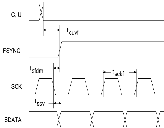
FSYNC Generated From Received Data
