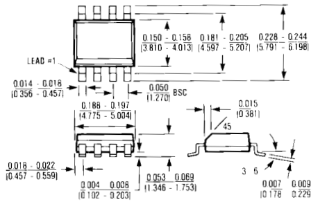
8 Lead Small Outline \theta_{JA} = 170 \text{ }^{\circ}\text{C/W} \theta_{JC} = 80 \text{ }^{\circ}\text{C/W}
