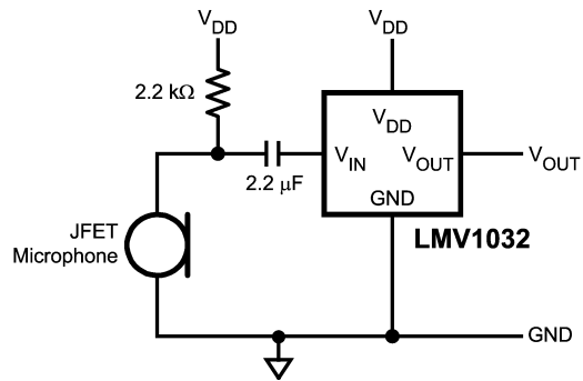
FIGURE 6. LMV1032 as External Pre-Amplifier
