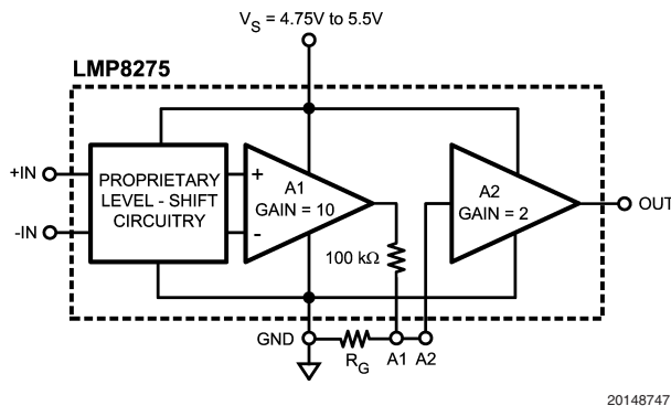
FIGURE 4. Gains Less Than 20
