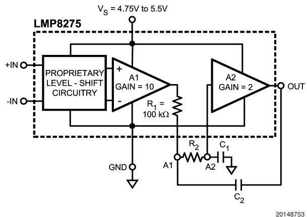
FIGURE 3. Low-Pass Filter With LMP8275
