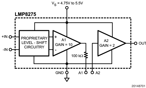
FIGURE 1. LMP8275
