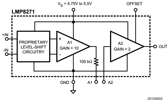
FIGURE 1. LMP8271
