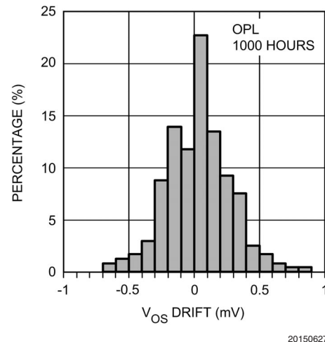
FIGURE 2. OPL Drift Histogram
