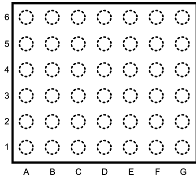
20100958 Top View (Bump Side Down) Order Number LM4931ITL See NS Package Number TLA42YVA
