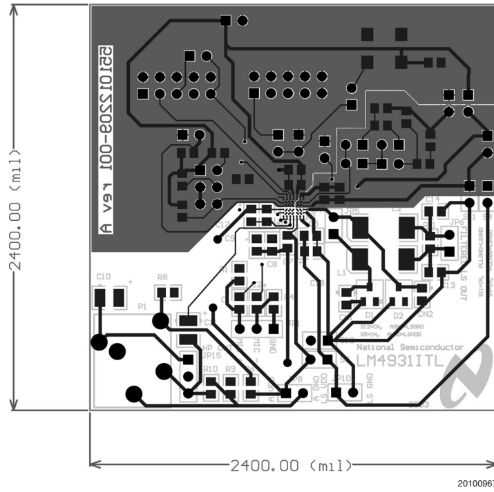
FIGURE 9. LM4931ITL Demo Board Composite View
