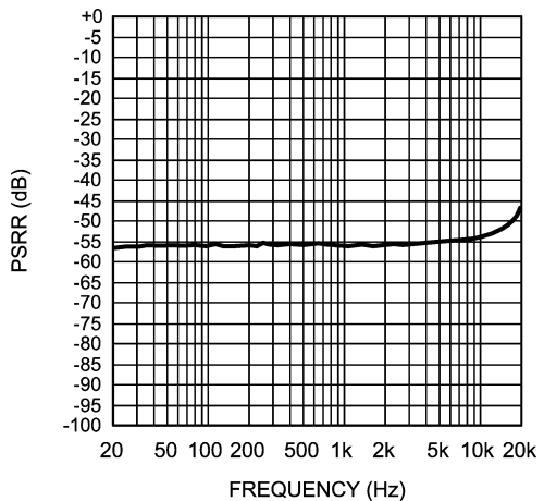
PSRR vs Frequency ( AV_{DD} = 3V , R_L = 8\Omega , Handsfree Output)
