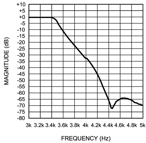
MIC PreAmp + ADC Frequency Response High Cutoff (MIC Gain = 36dB)
