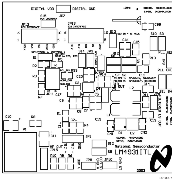
FIGURE 10. LM4931ITL Demo Board Silkscreen
