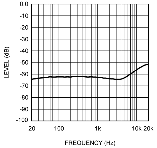
PSRR vs Frequency V_{DD} = 1.8V, R_L = 16\Omega
