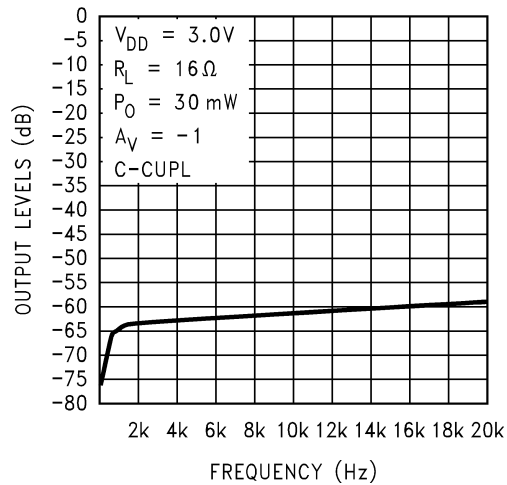
Channel Separation
