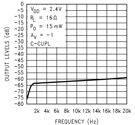
Channel Separation
