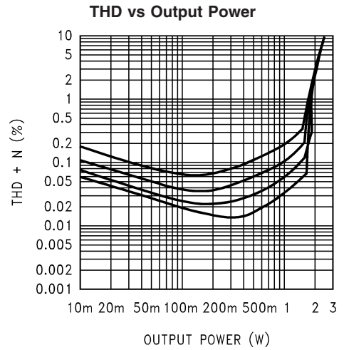
201163A1 V_{DD} = 5V , R_L = 4\Omega , f_{IN} = 1kHz , at (from top to bottom at 200mW): A_V = 21.6dB , A_V = 15.6dB , A_V = 10dB , A_V = 6dB
