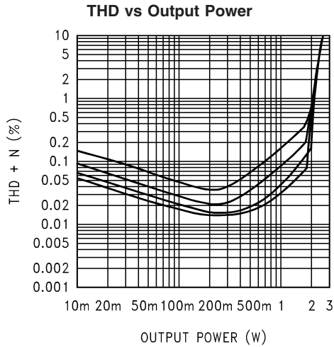
20116344 V_{DD} = 5V , R_L = 3\Omega , f_{IN} = 1kHz , at (from top to bottom at 50mW): A_V = 21.6dB , A_V = 15.6dB , A_V = 10dB , A_V = 6dB
