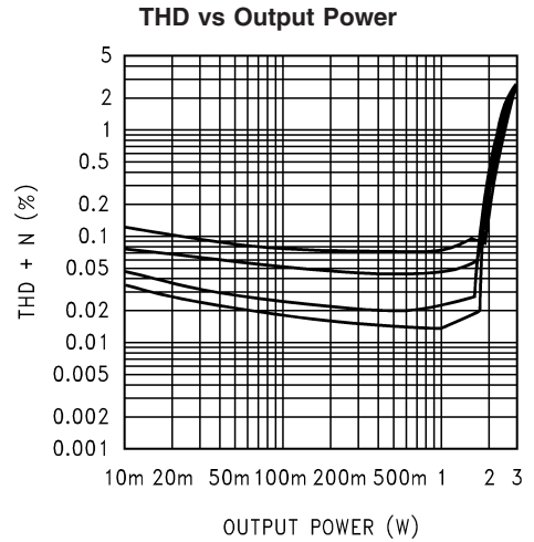
20116345 V_{DD} = 5V , R_L = 3\Omega , f_{IN} = 20kHz , at (from top to bottom at 50mW): A_V = 21.6dB , A_V = 15.6dB , A_V = 10dB , A_V = 6dB
