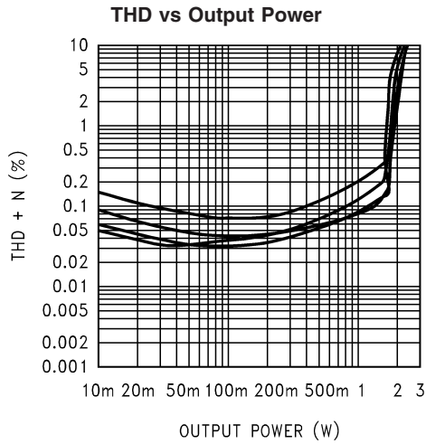
201163A0 V_{DD} = 5V , R_L = 4\Omega , f_{IN} = 20Hz , at (from top to bottom at 100mW): A_V = 21.6dB , A_V = 15.6dB , A_V = 6dB , A_V = 10dB
