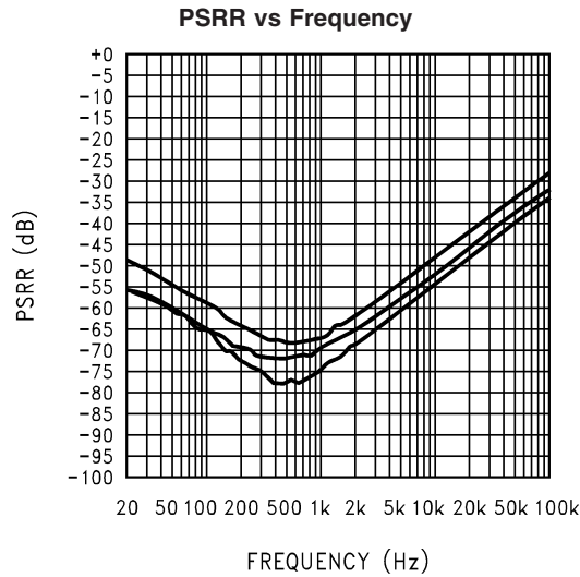
20079726 V_{DD} = 5V ; LLS, RLS; R_L = 8\Omega ; 0db Gain; All audio inputs terminated Top-Mode 12, 13; Mid-Mode 2, 3; Bot-Mode 7, 8
