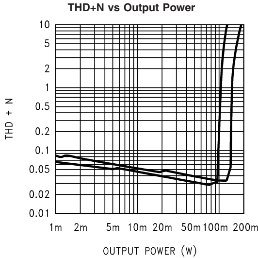
20079724 V_{DD} = 5V ; EP; f = 1kHz ; R_L = 32\Omega ; Mode 1; 0dB Gain; Top-CD4 = 1; Bot-CD4 = 0
