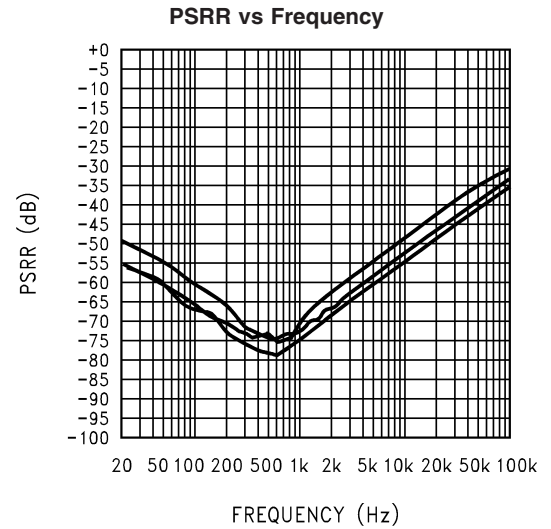
20079727 V_{DD} = 3V ; LLS, RLS; R_L = 8\Omega ; 0db Gain; All audio inputs terminated Top-Mode 12, 13; Mid-Mode 2, 3; Bot-Mode 7, 8
