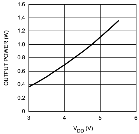
Output Power vs Supply Voltage R_L = 8\Omega , Mode 1
