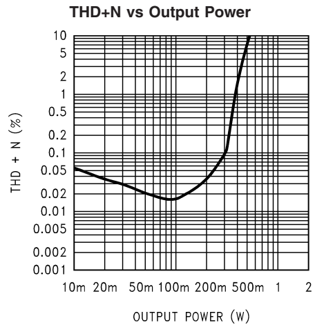
20078128 V_{DD} = 3V, R_L = 8\Omega, f_{IN} = 1kHz
