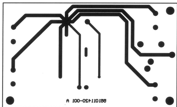
FIGURE 5. Recommended PC Board Layout Bottom-Side Layout
