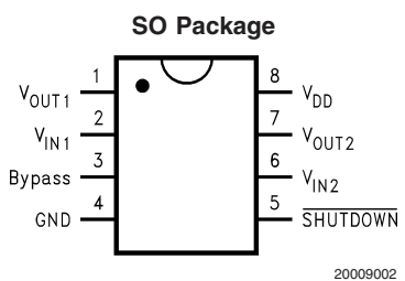
Top View Order Number LM4809MA See NS Package Number M08A
