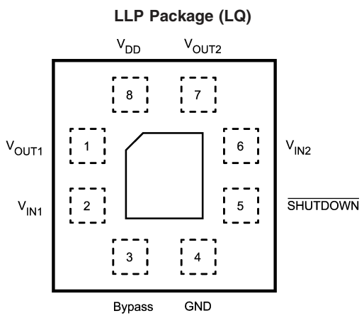
Top View Order Number LM4809LQ See NS Package Number LQB08A
