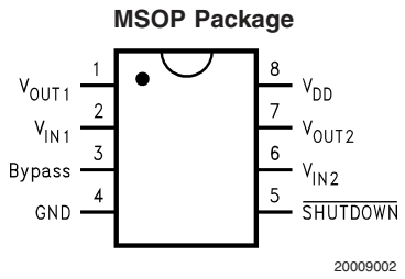
Top View Order Number LM4809MM See NS Package Number MUA08A
