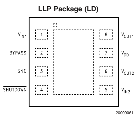
Top View Order Number LM4809LD See NS Package Number LDA08B
