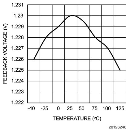
Feedback Voltage vs Temperature
