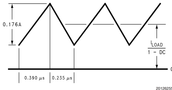
FIGURE 2. 10µH Inductor Current 5V - 12V Boost (LM4805)
