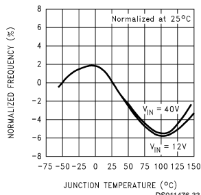
Oscillator Frequency
