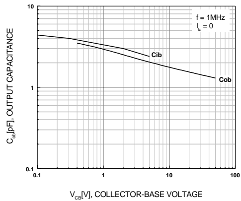
Figure 6. Output Capacitance
