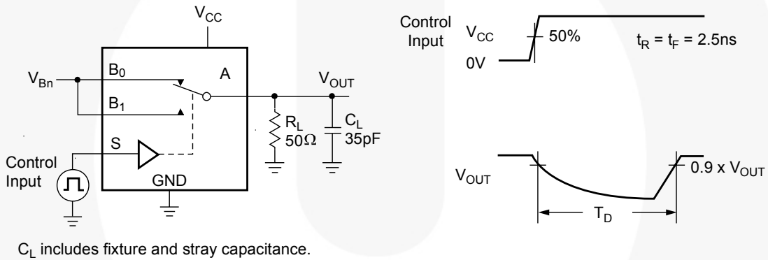
Figure 12. Break-Before-Make Timing
