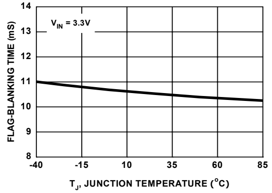
Figure 14. T_{\text{BLANK}} vs. Temperature
