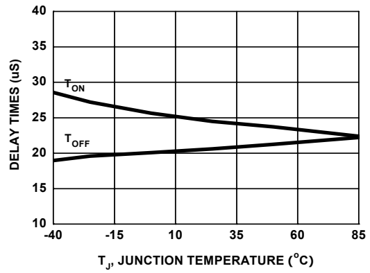
Figure 12. T ON /T OFF vs. Temperature
