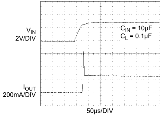
Figure 19. Current Limit Response Time (Switch power up to hard short)
