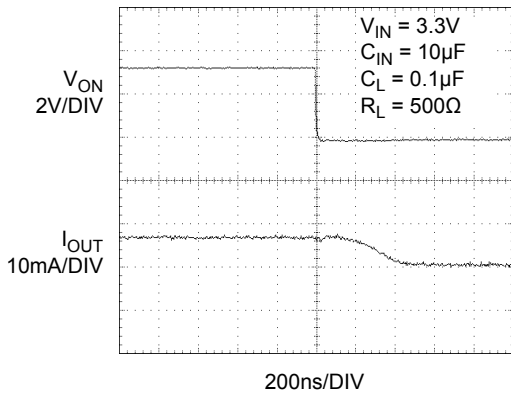
Figure 17. T_{\text{OFF}} Response
