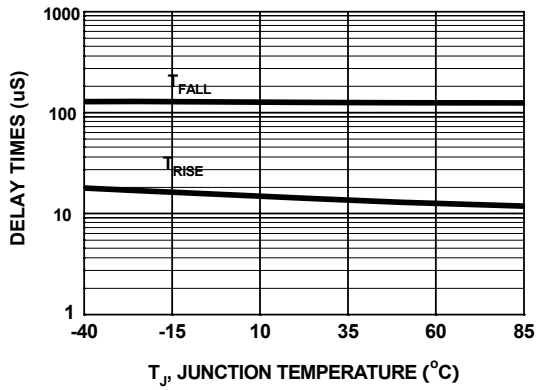
Figure 13. T_{\text{Rise}}/T_{\text{Fall}} vs. Temperature
