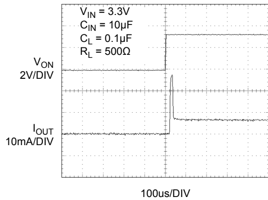
Figure 16. T_{\text{ON}} Response
