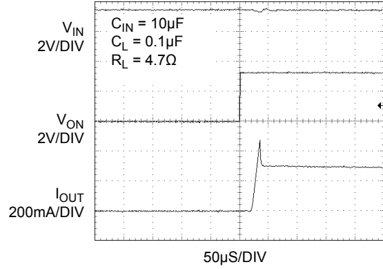
Figure 20. Current Limit Response Time (Output has a 4.7Ω load)
