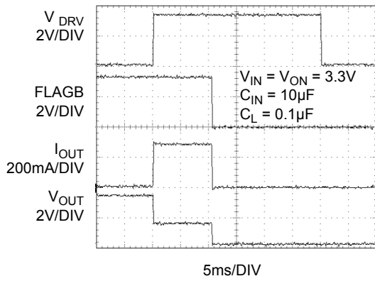
Figure 15. T_{\text{BLANK}} Response
