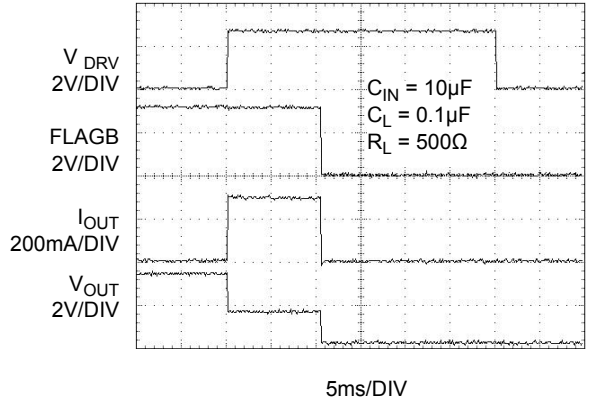
Figure 14. T_{BLANK} Response
