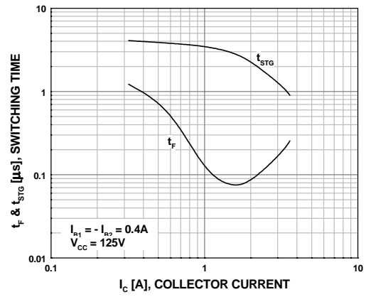
Figure 8. Switching Time
