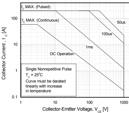
Fig 11. SOA Characteristics
