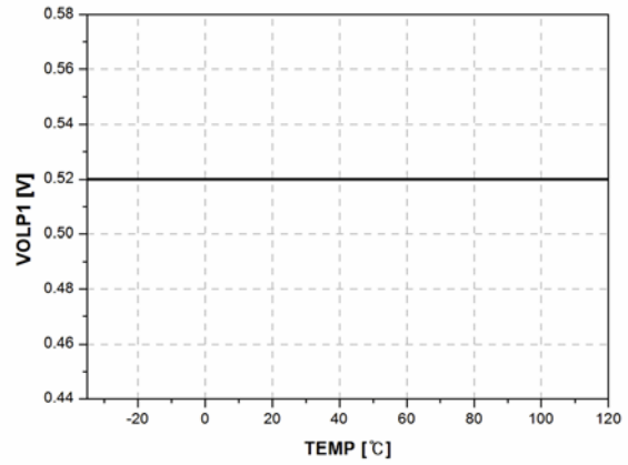
Figure 34. Open-Lamp Protection Voltage1 vs. Temp.
