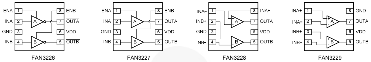
Figure 4. Pin Configurations (Repeated)
